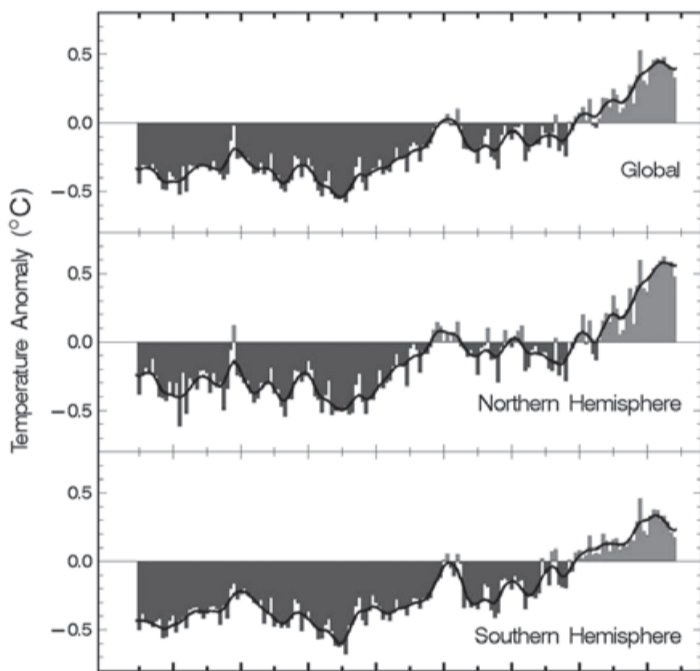
Global and Hemispheric Annual Temperature Anomalies 1850—2008
